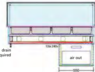
work top cutout 1380W x 680D
