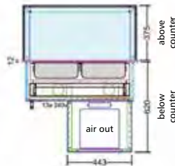
work top cutout 750W x 680D
