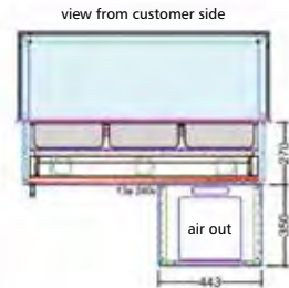
work top cutout 1050W x 680D
